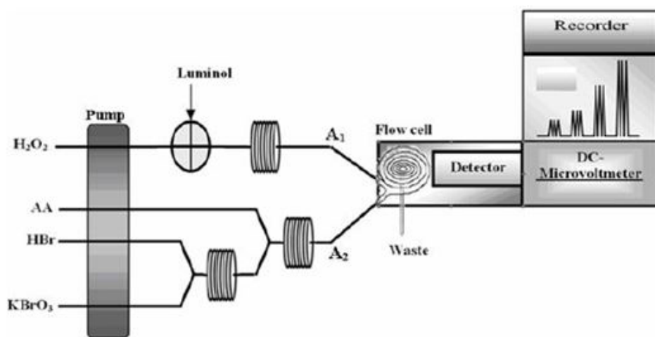
Figure 1: Schematic Diagram of the rFIA-CL Manifold used in this Study for the Determination of Ascorbic Acid
